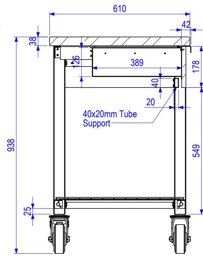
SECTION B-B
